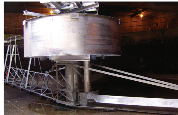
Riser Pipe Clarifiers can be converted to a Tow-Bro® Clarifier Hydraulic Removal System
